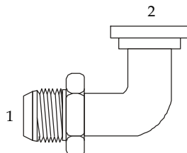
(1) Male Tube (2) C 61 Flange
