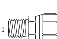
(1) Male Face Seal (2) Female JIC
