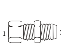
(1) Female NPT (2) JIC Bulkhead
