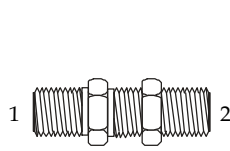
(1) Male Face Seal (2) Face Seal Bulkhead
