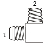
(1) Male JIC (2) Male NPT
