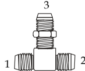
(1)(2) Male JIC (3) JIC Bulkhead
