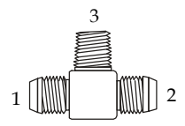
(1) (2) Male JIC (2) Male NPT
