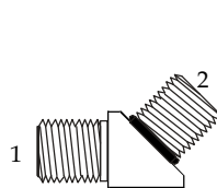
(1) Male Face Seal (2) Male Adj. ORB
