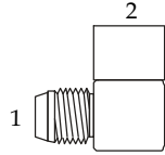
(1) Male JIC (2) Female NPT
