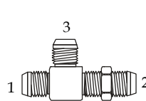
(1)(3) Male JIC (2) JIC Bulkhead
