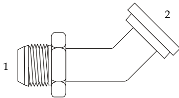
(1) Male Tube (2) C 61 Flange
