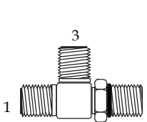
(1)(3) Male Face Seal (2) Male Adj. ORB
