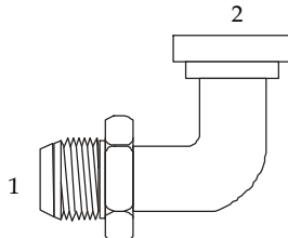
(1) Male Tube (2) C 62 Flange
